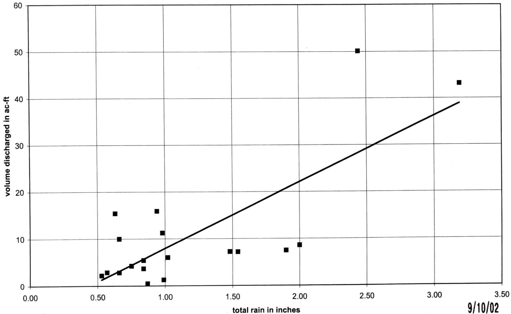
Figure 7 - Conard Branch 2001 Storm Set
